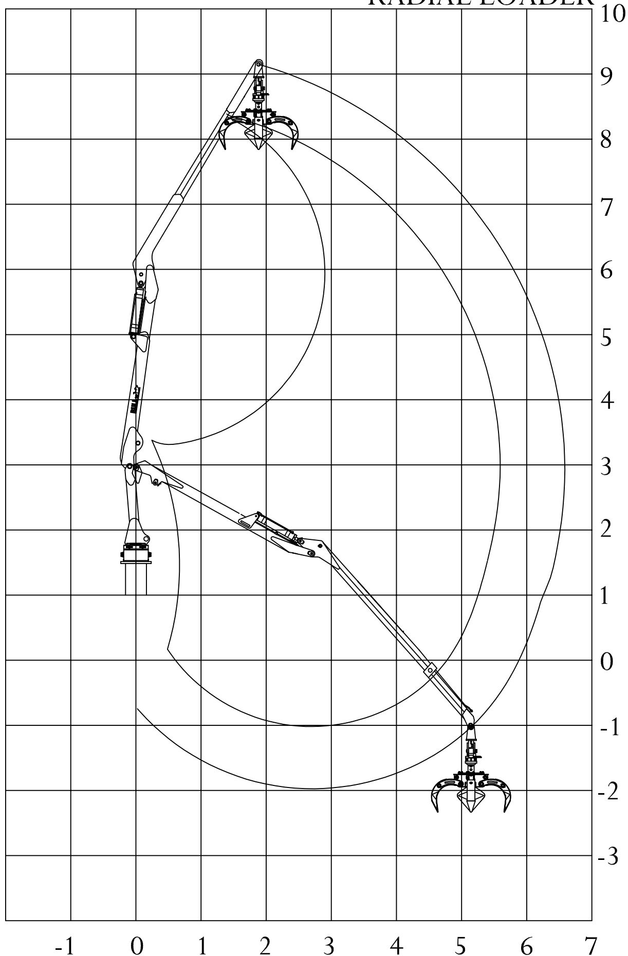
LIFTING AND DIGGING DIAGRAM FOR TELESCOPIC RADIAL LOADER (All dimensions in metre.)
